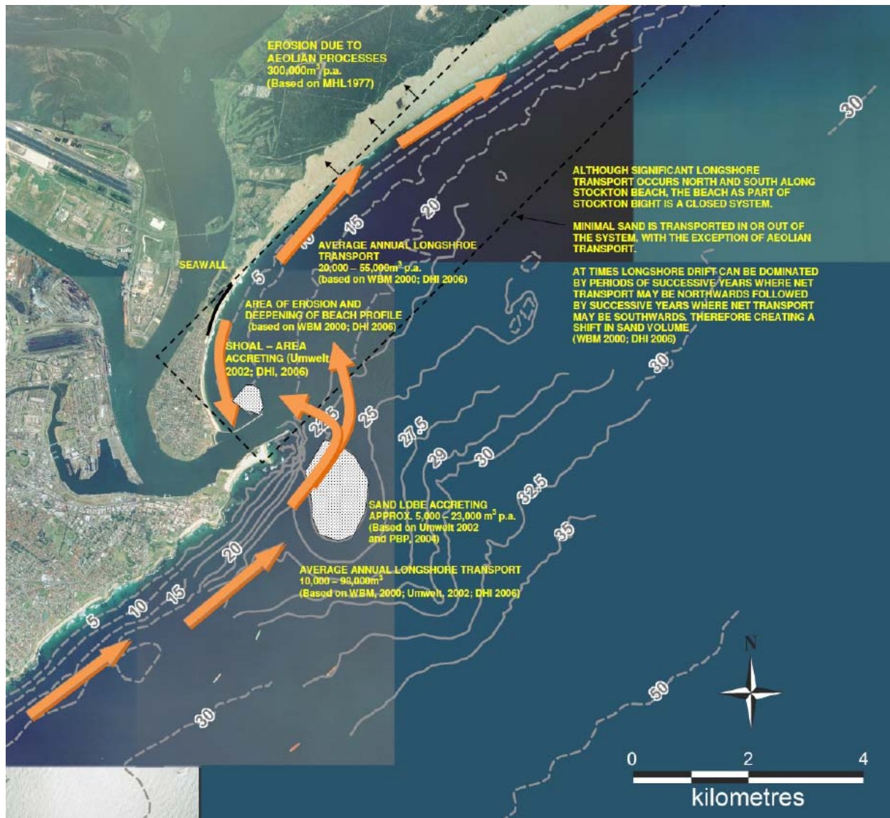
Figure 3: Conceptual sediment processes model developed as part of the Stockton Beach Sand Scoping Study (Worely Parsons, 2012)
