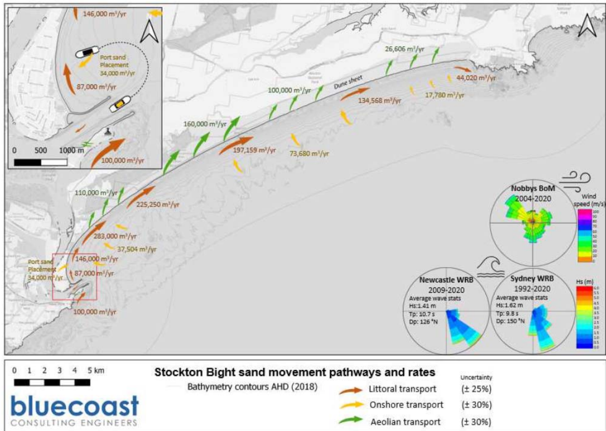
Figure 4: Conceptual sand movement model developed by Bluecoast (2020)
