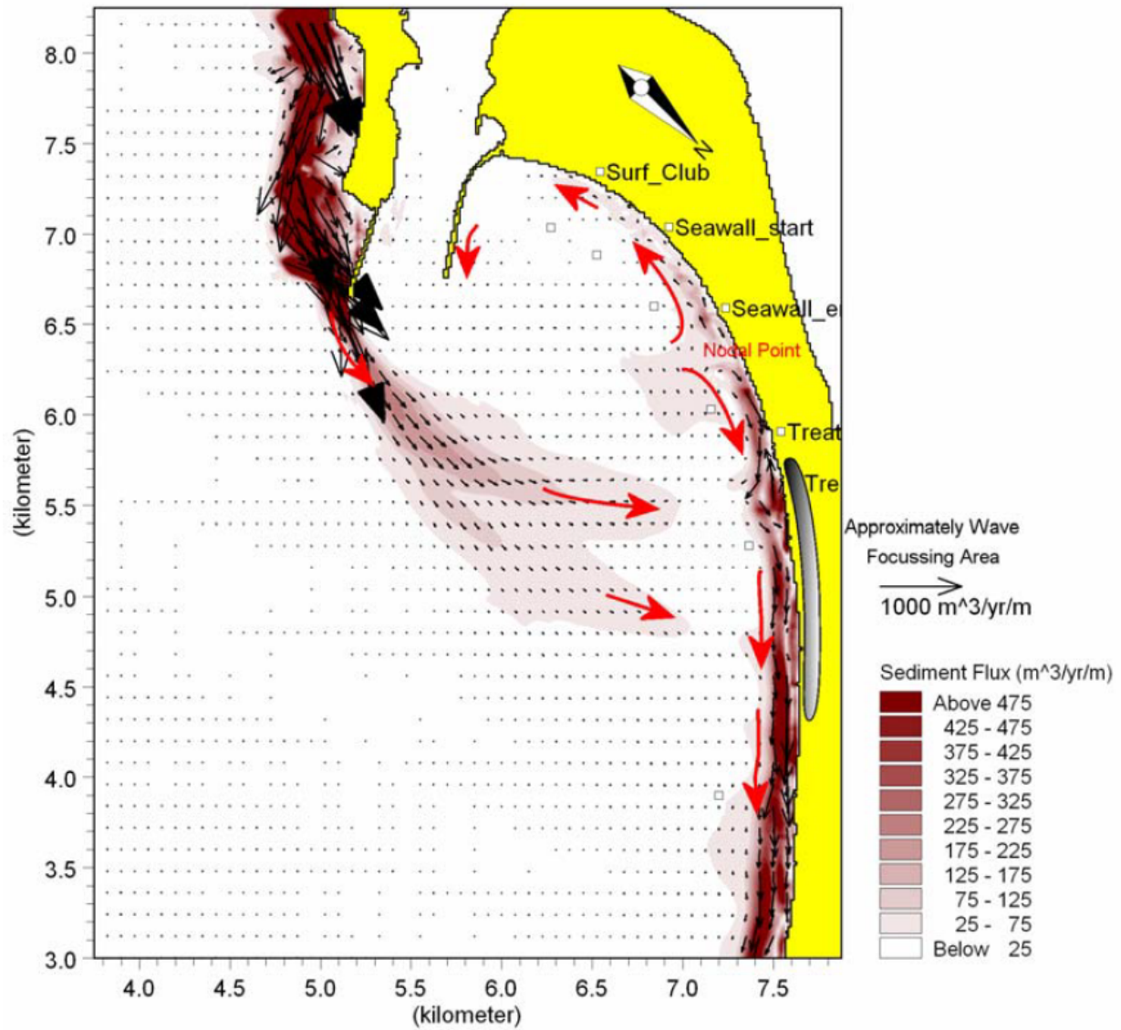
Figure 2: The predicted sediment transport mechanisms at Stockton based on the typical yearly conditions from 1992 to 2005. (DHI, 2006)
